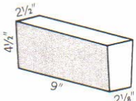
No. 1 Arch 9 x 4 1/2 x (2 1/2 - 2 1/8)" 9" Eq.—0.92
