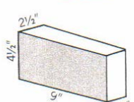
No. 1 Wedge 9 x 4 1/2 x (2 1/2 - 1 7/8)" 9" Eq.—0.87
