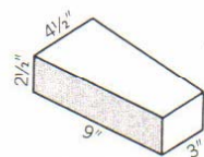
No. 3 Key 9 x (4 1/2 - 3) x 2 1/2" 9" Eq.—0.83
