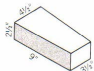
No. 2 Key 9 x (4 1/2 - 3 1/2) x 2 1/2" 9" Eq.—0.89
