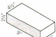
No. 1 Key 9 x (4 1/2 - 4) x 2 1/2" 9" Eq.—0.94
