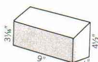
60° Side Skew 9 x (4 1/2 - 3 1/8) x 2 1/2" 9" Eq.—0.84
