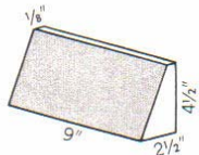
Featheredge 9 x 4 1/2 x (2 1/2 - 1/8)" 9" Eq.—0.52
