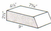
60° End Skew (9 - 7 1/8) x 4 1/2 x 2 1/2" 9" Eq.—0.92
