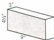
No. 2 Split (2") † 9 x 4 1/2 x 2" 9" Eq.—0.80
