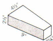
No. 4 Key 9 x (4 1/2 - 2 1/4) x 2 1/2" 9" Eq.—0.75
