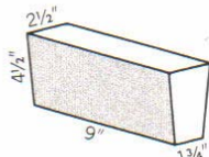
No. 2 Arch 9 x 4 1/2 x (2 1/2 - 1 3/4)" 9" Eq.—0.85
